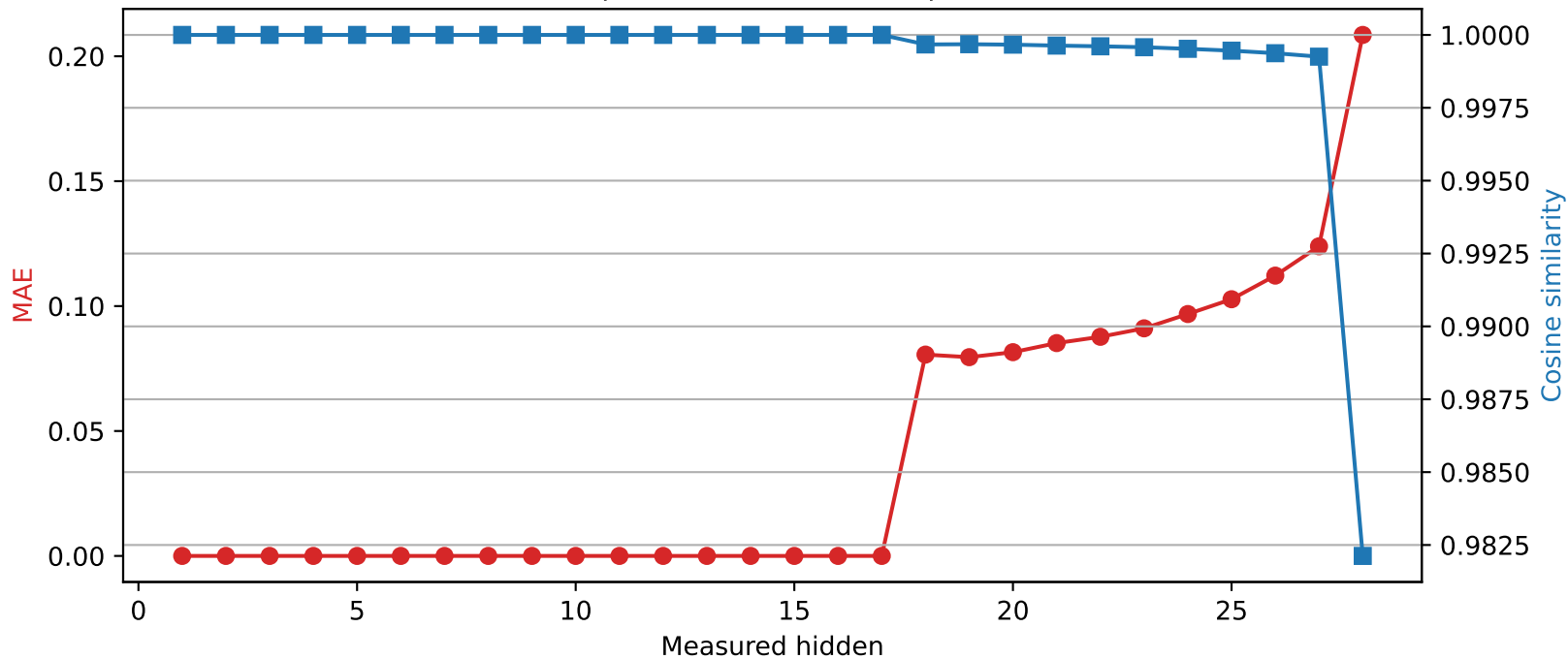
Llama-3.2-3B | Quantized layer 17 | float32 → int4
