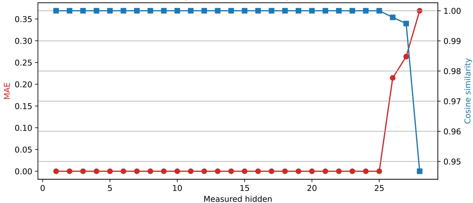
Llama-3.2-3B | Quantized layer 25 | float32 \rightarrow int4
