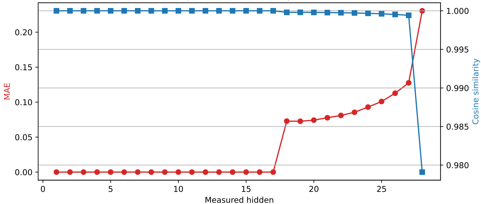
Llama-3.2-3B | Quantized layer 17 | float64 → int4
