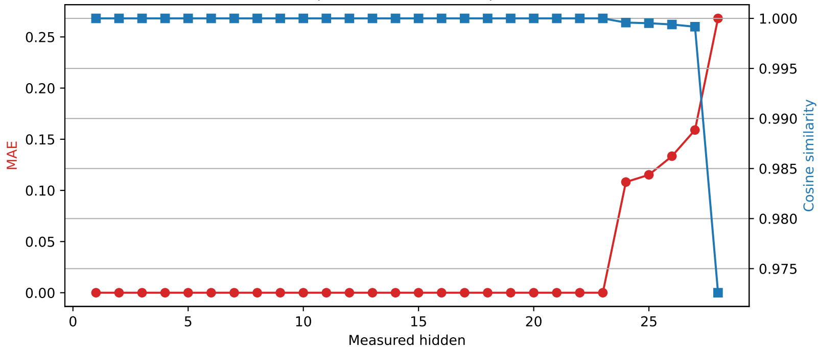
Llama-3.2-3B | Quantized layer 23 | float64 → int4
