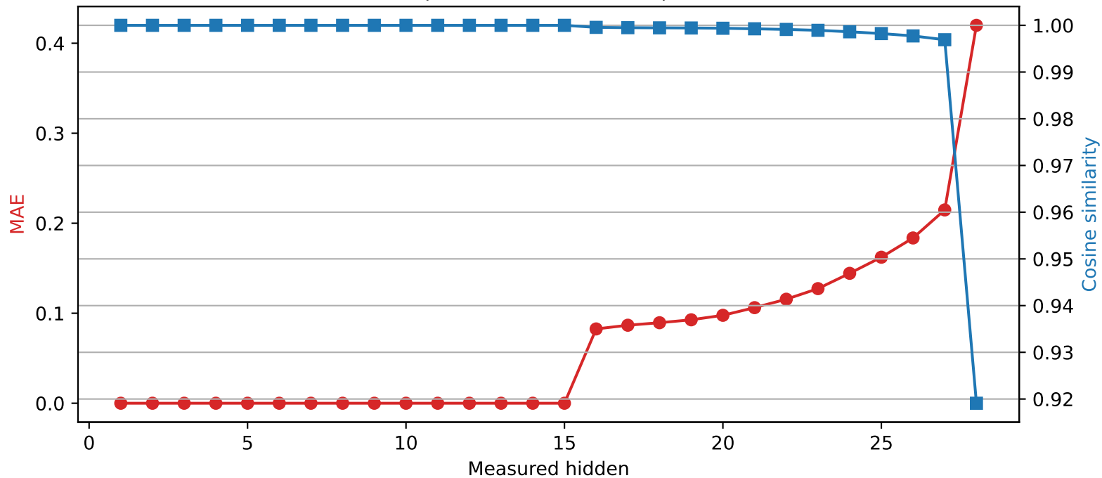
Llama-3.2-3B | Quantized layer 15 | float64 → int4
