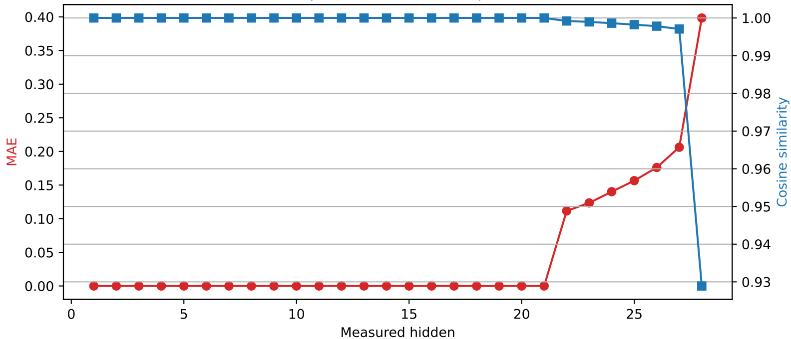
Llama-3.2-3B | Quantized layer 21 | float64 → int4
