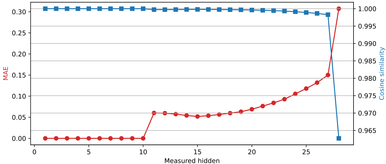
Llama-3.2-3B | Quantized layer 10 | float64 → int4
