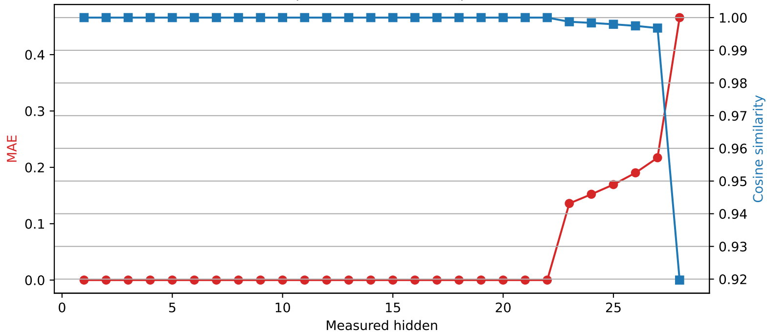
Llama-3.2-3B | Quantized layer 22 | float64 → int4
