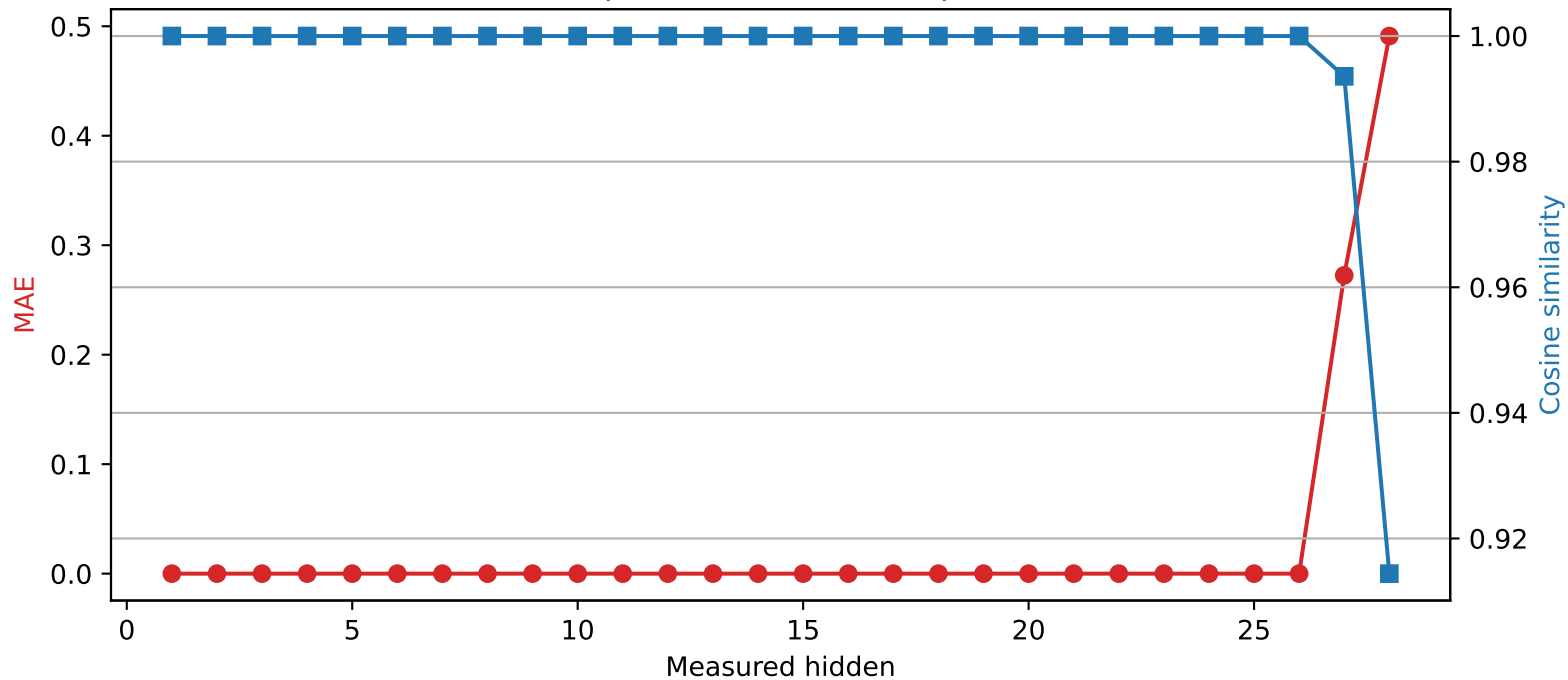
Llama-3.2-3B | Quantized layer 26 | float64 → int4
