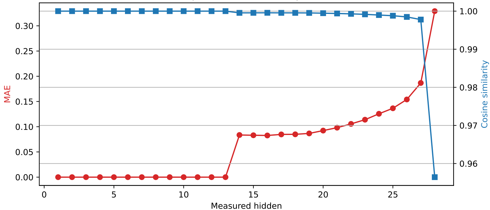
Llama-3.2-3B | Quantized layer 13 | float64 → int4
