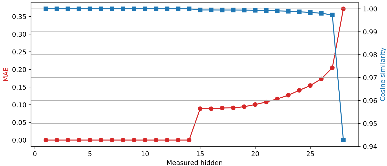
Llama-3.2-3B | Quantized layer 14 | float64 → int4
