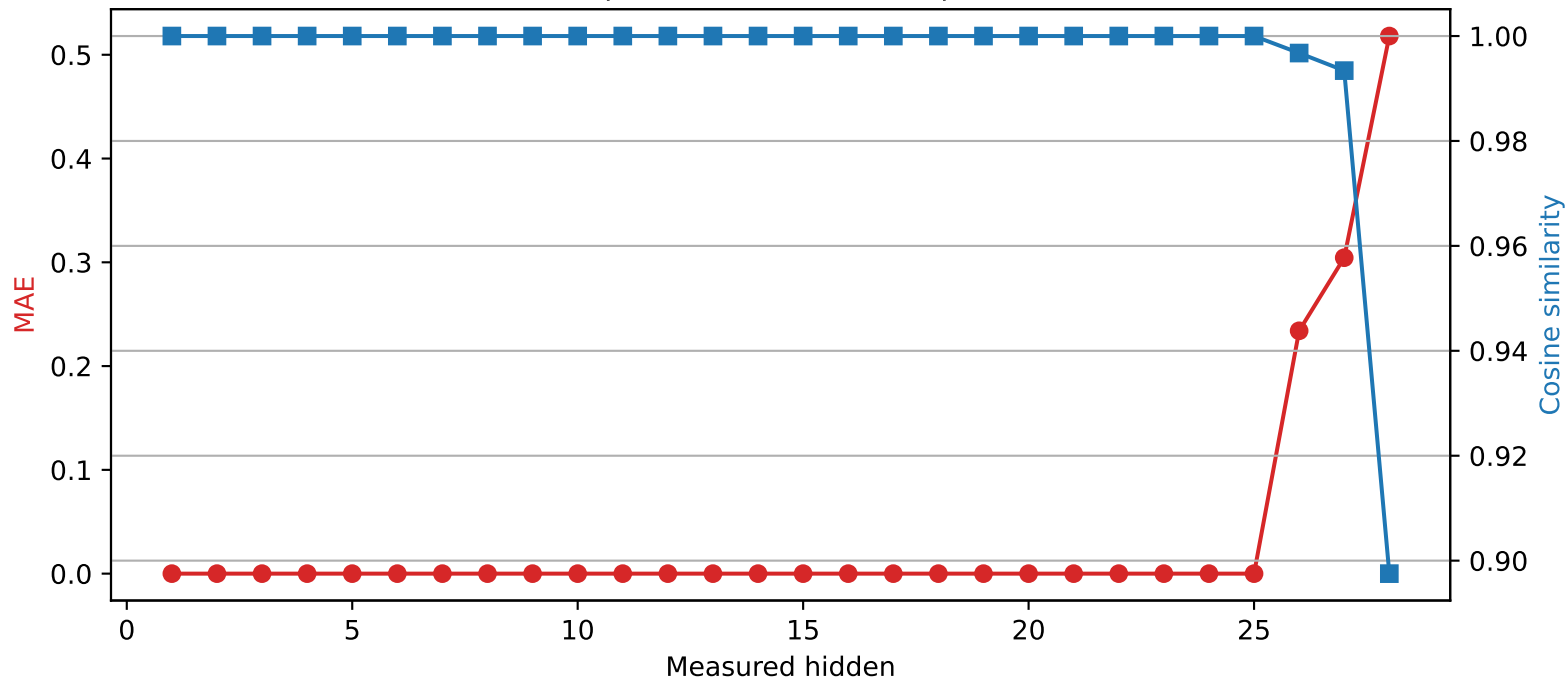
Llama-3.2-3B | Quantized layer 25 | float64 → int4
