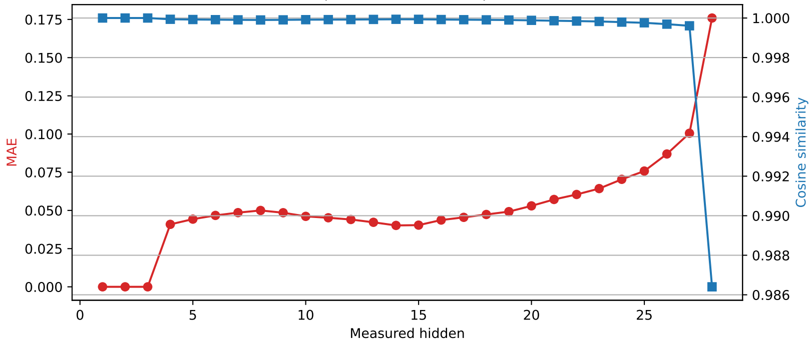
Llama-3.2-3B | Quantized layer 3 | float16 → int2
