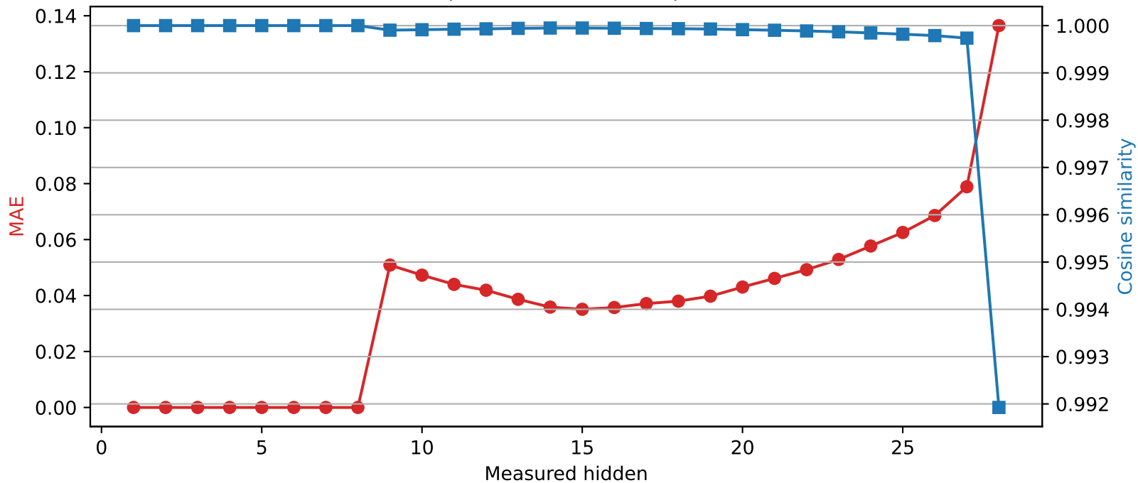
Llama-3.2-3B | Quantized layer 8 | float16 → int2
