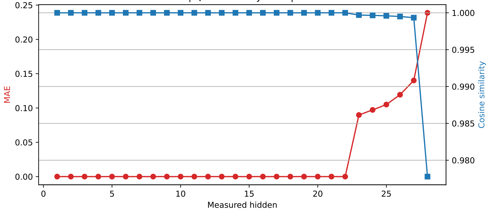
Llama-3.2-3B | Quantized layer 22 | float16 \rightarrow int2
