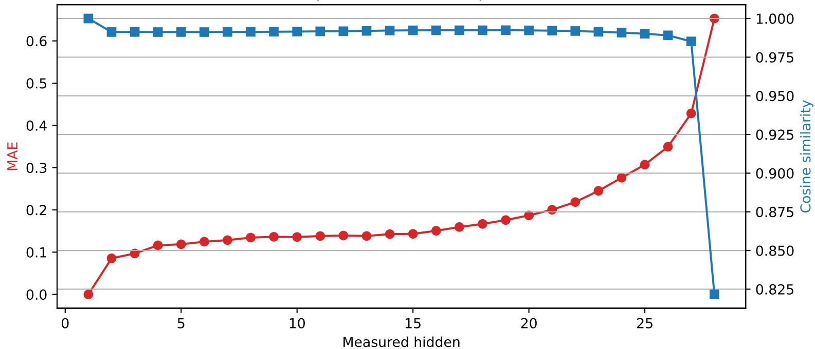
Llama-3.2-3B | Quantized layer 1 | float16 → int2
