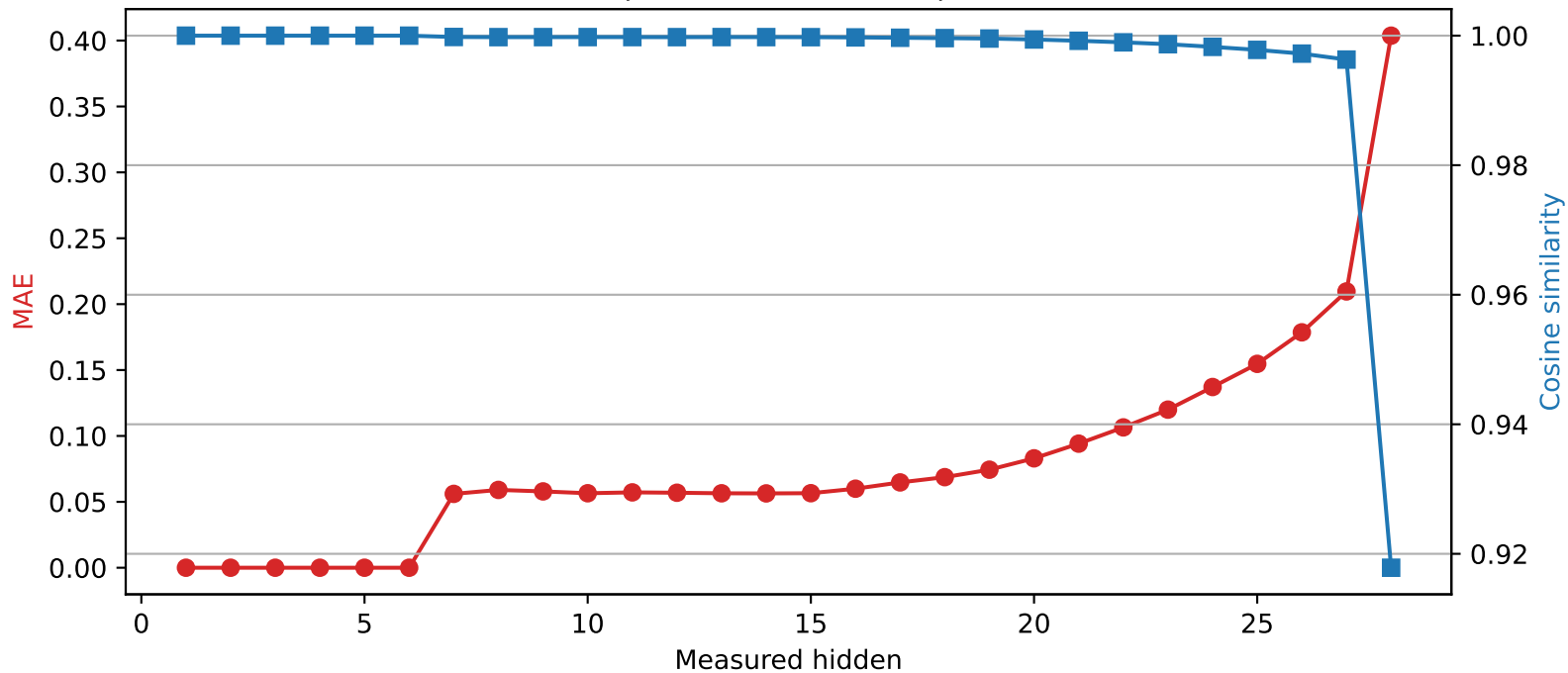
Llama-3.2-3B | Quantized layer 6 | float16 → int2
