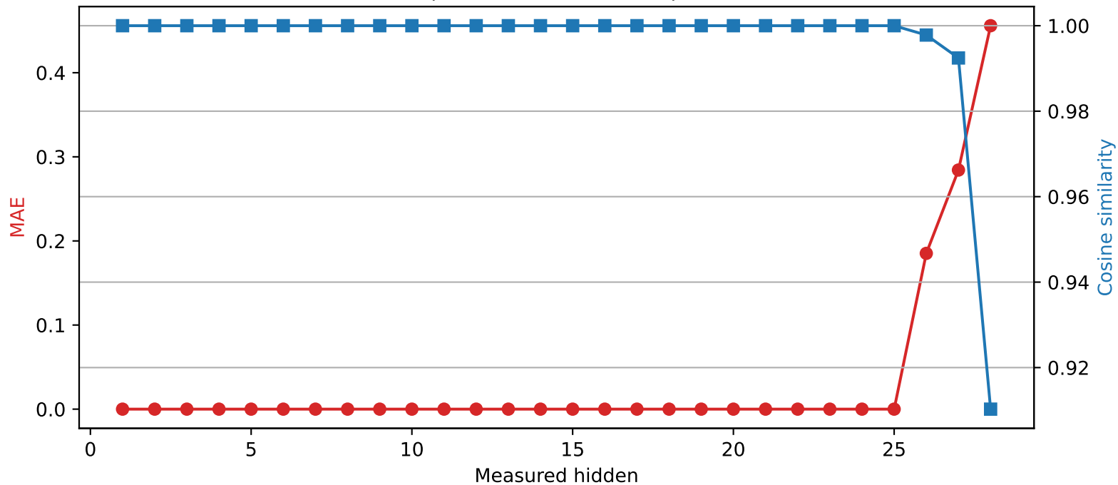
Llama-3.2-3B | Quantized layer 25 | float16 → int2
