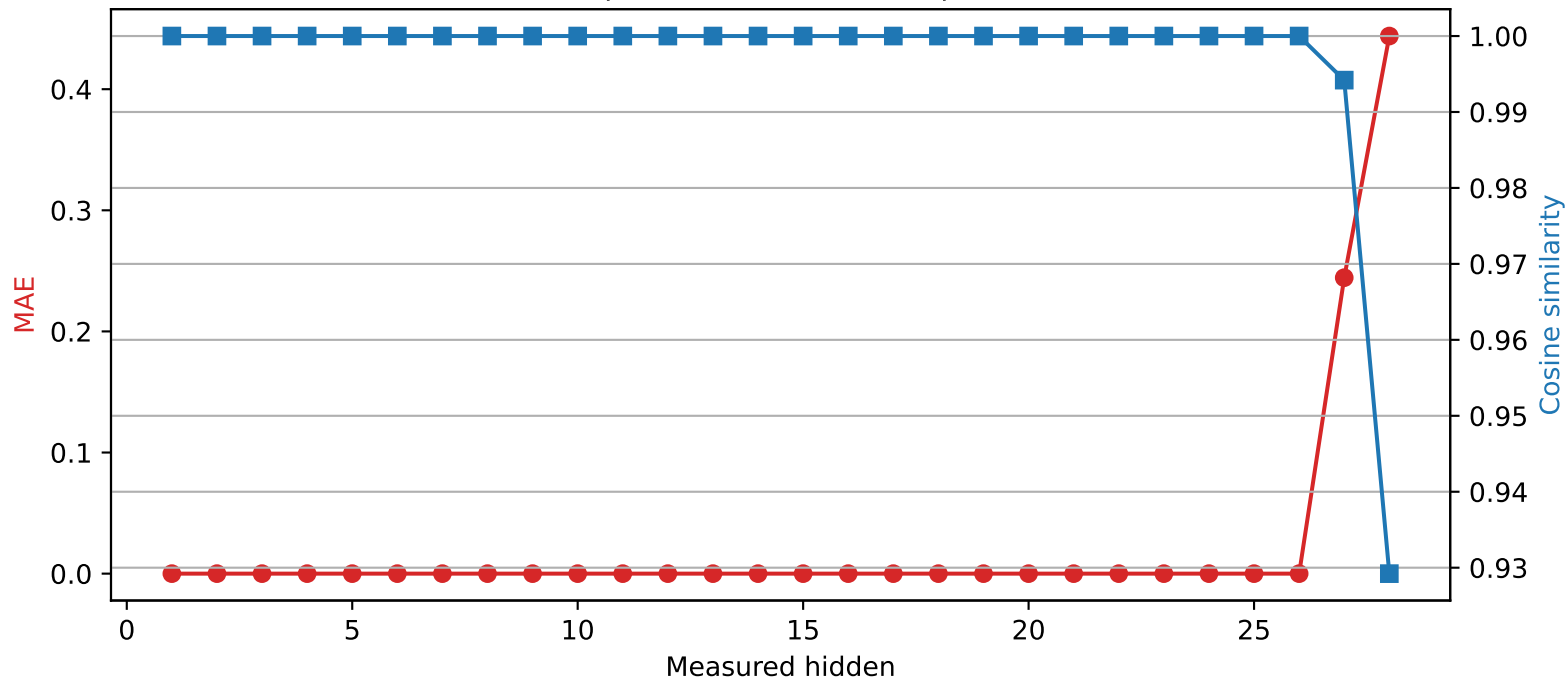
Llama-3.2-3B | Quantized layer 26 | float16 → int2
