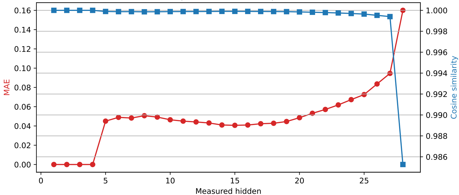
Llama-3.2-3B | Quantized layer 4 | float16 → int2
