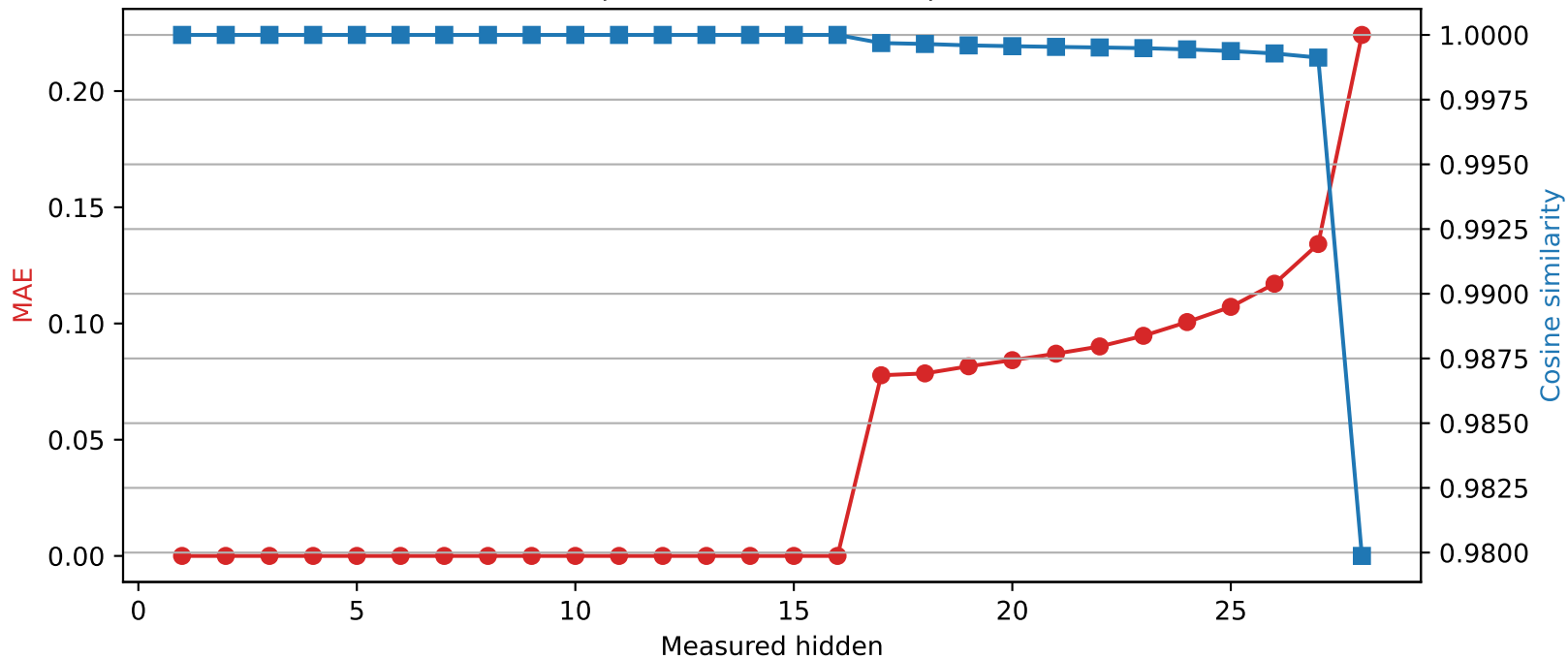
Llama-3.2-3B | Quantized layer 16 | float16 → int2
