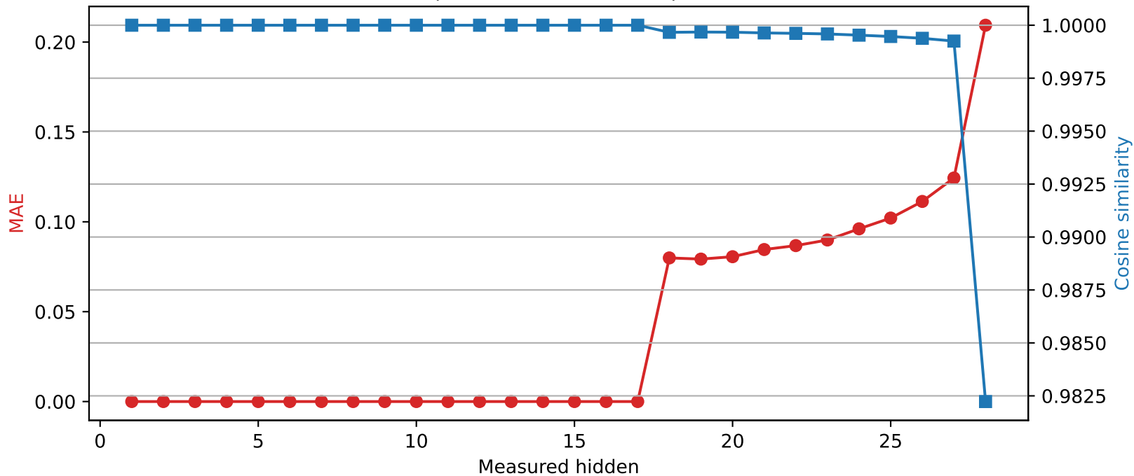
Llama-3.2-3B | Quantized layer 17 | float16 → int2
