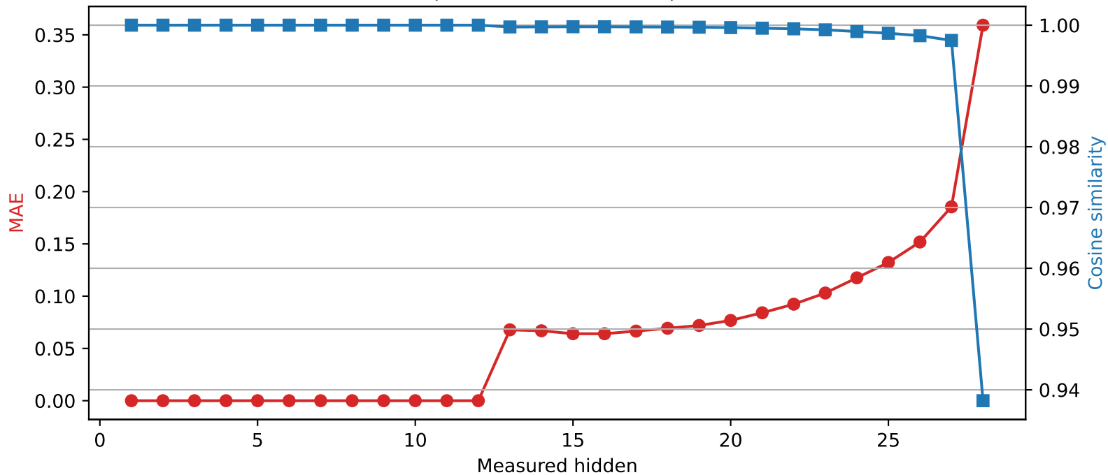
Llama-3.2-3B | Quantized layer 12 | float32 → int2
