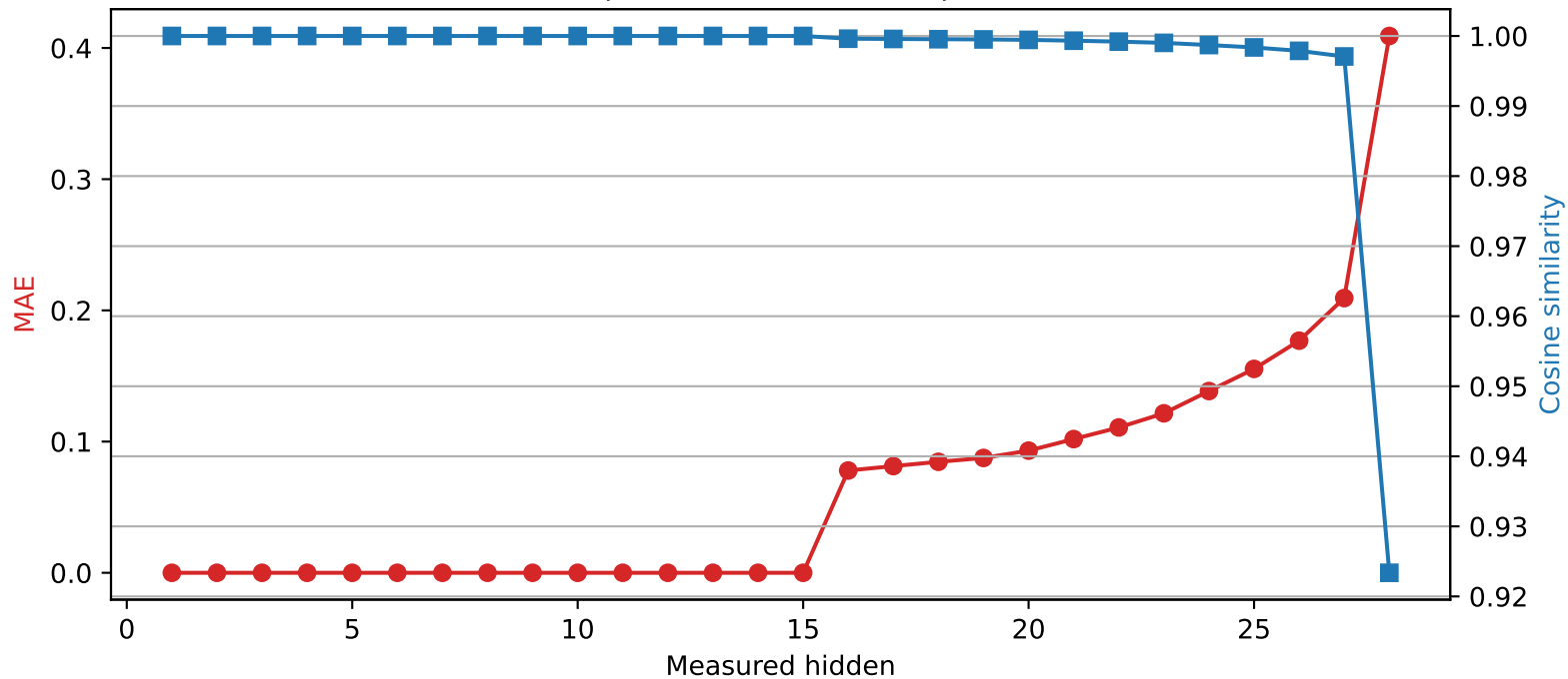
Llama-3.2-3B | Quantized layer 15 | float32 → int2
