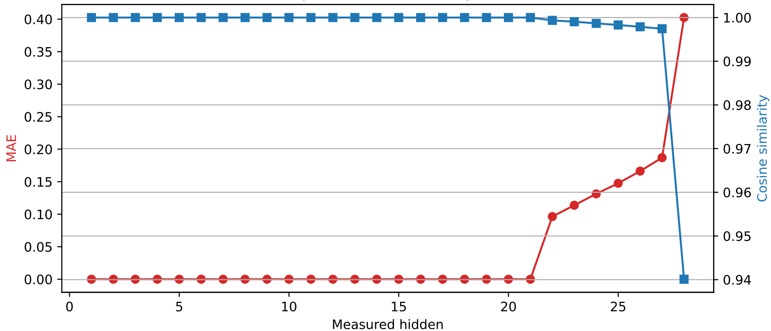
Llama-3.2-3B | Quantized layer 21 | float32 → int2
