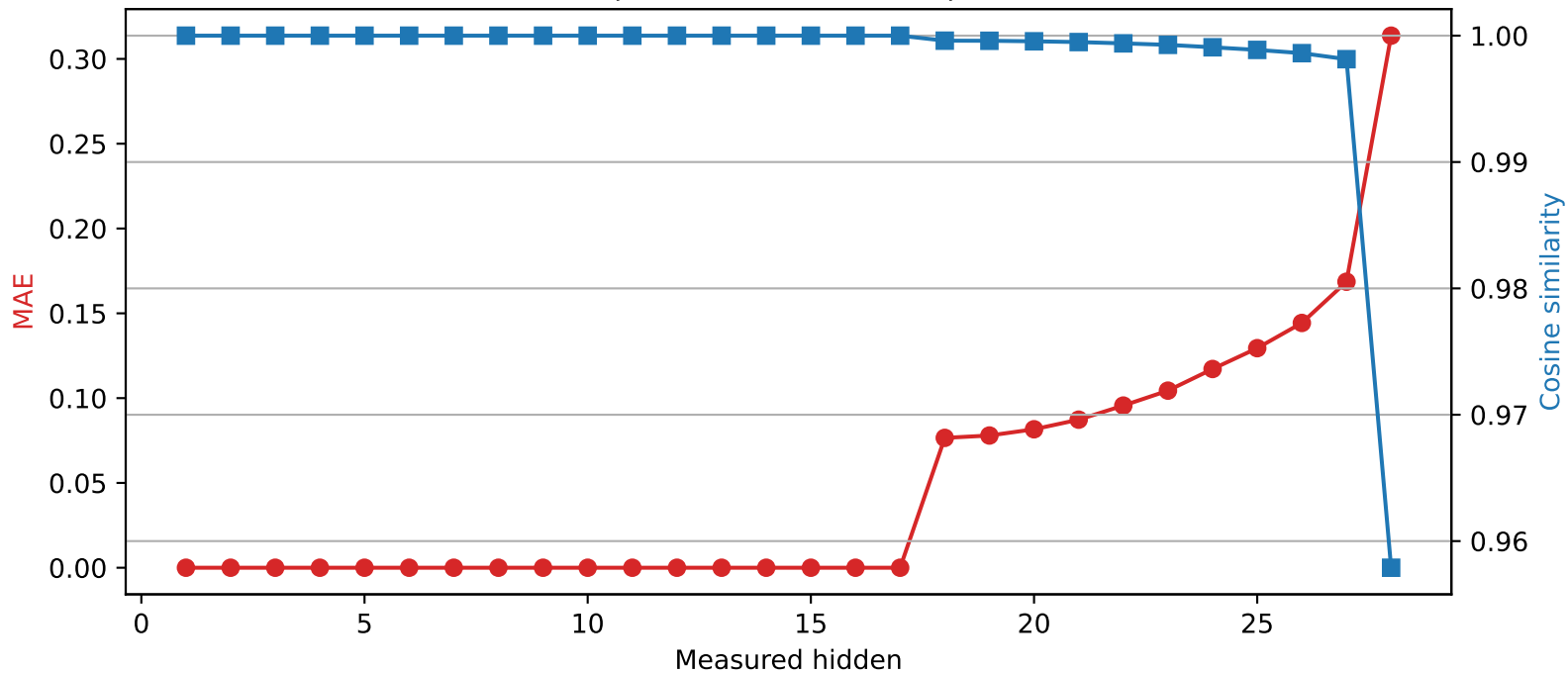
Llama-3.2-3B | Quantized layer 17 | float32 → int2
