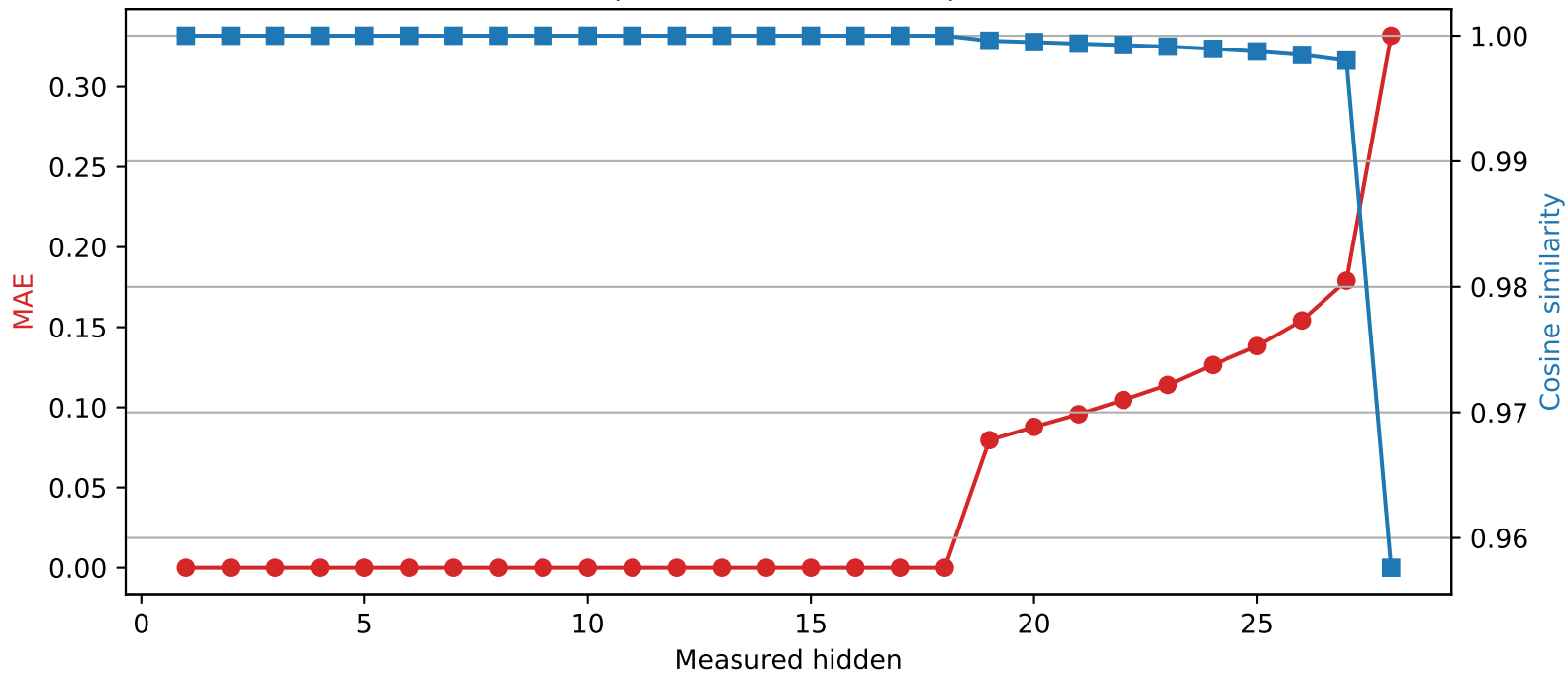
Llama-3.2-3B | Quantized layer 18 | float32 → int2
