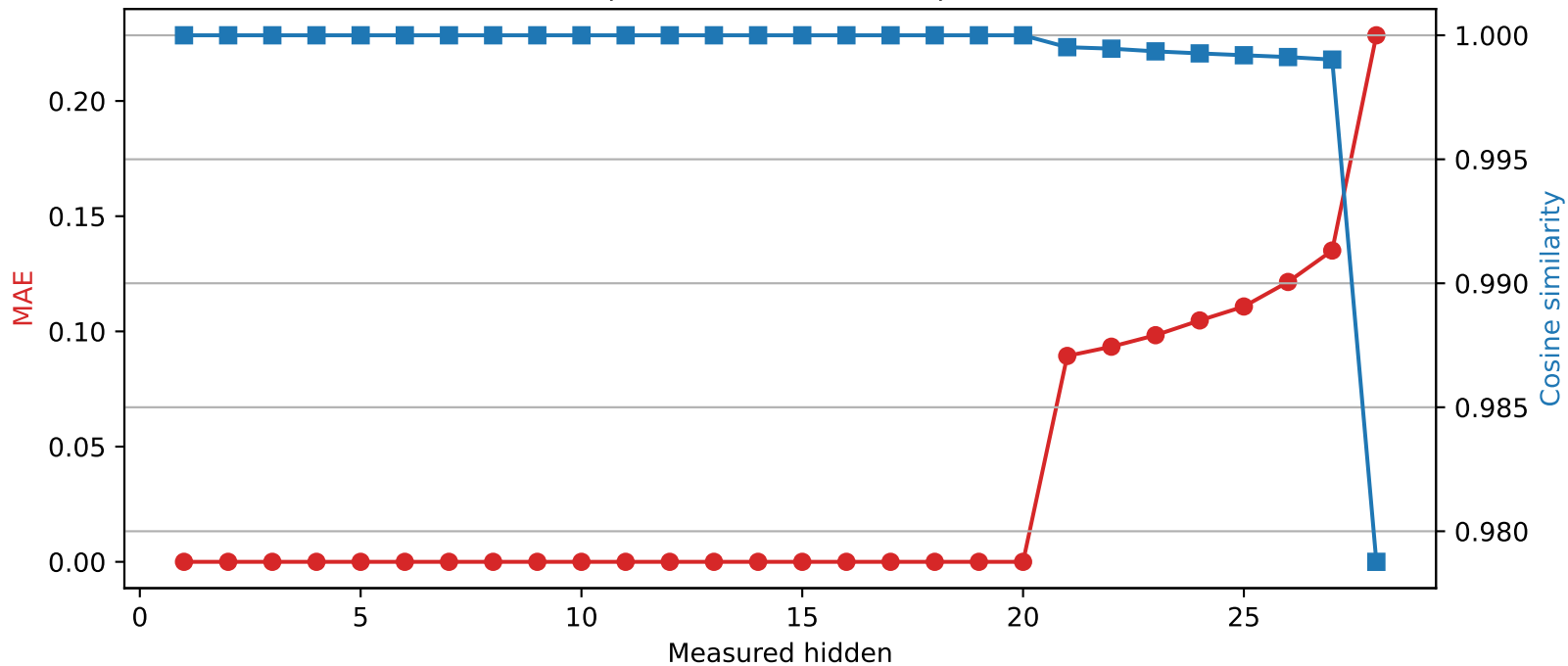
Llama-3.2-3B | Quantized layer 20 | float32 → int2
