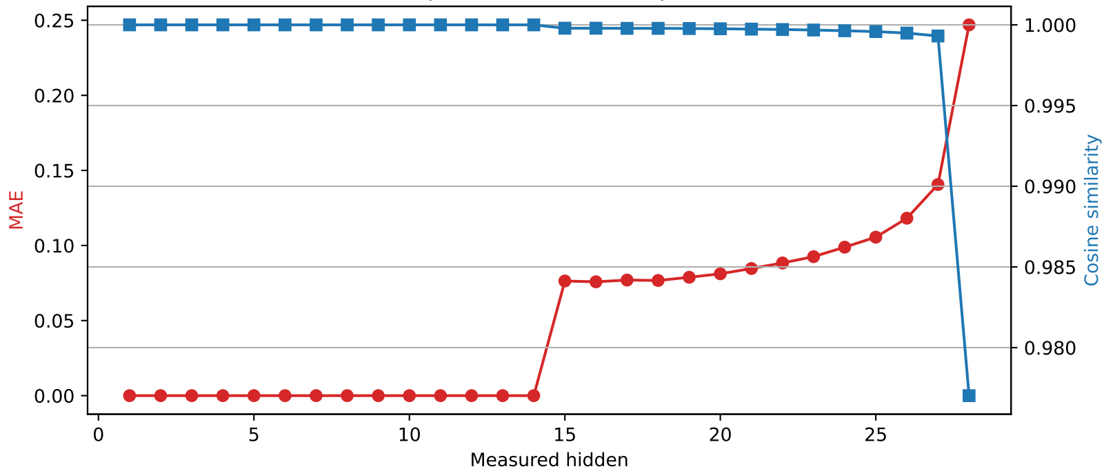
Llama-3.2-3B | Quantized layer 14 | float64 → int2
