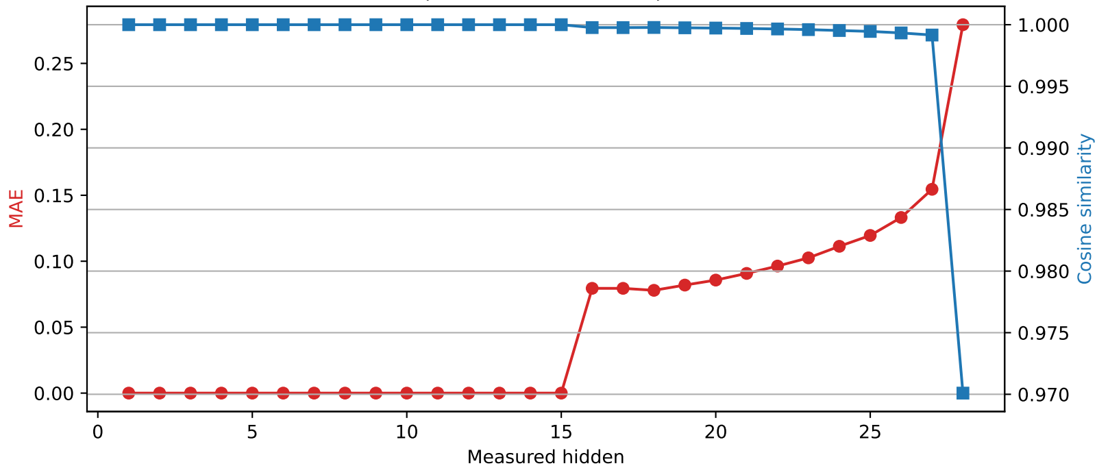
Llama-3.2-3B | Quantized layer 15 | float64 → int2
