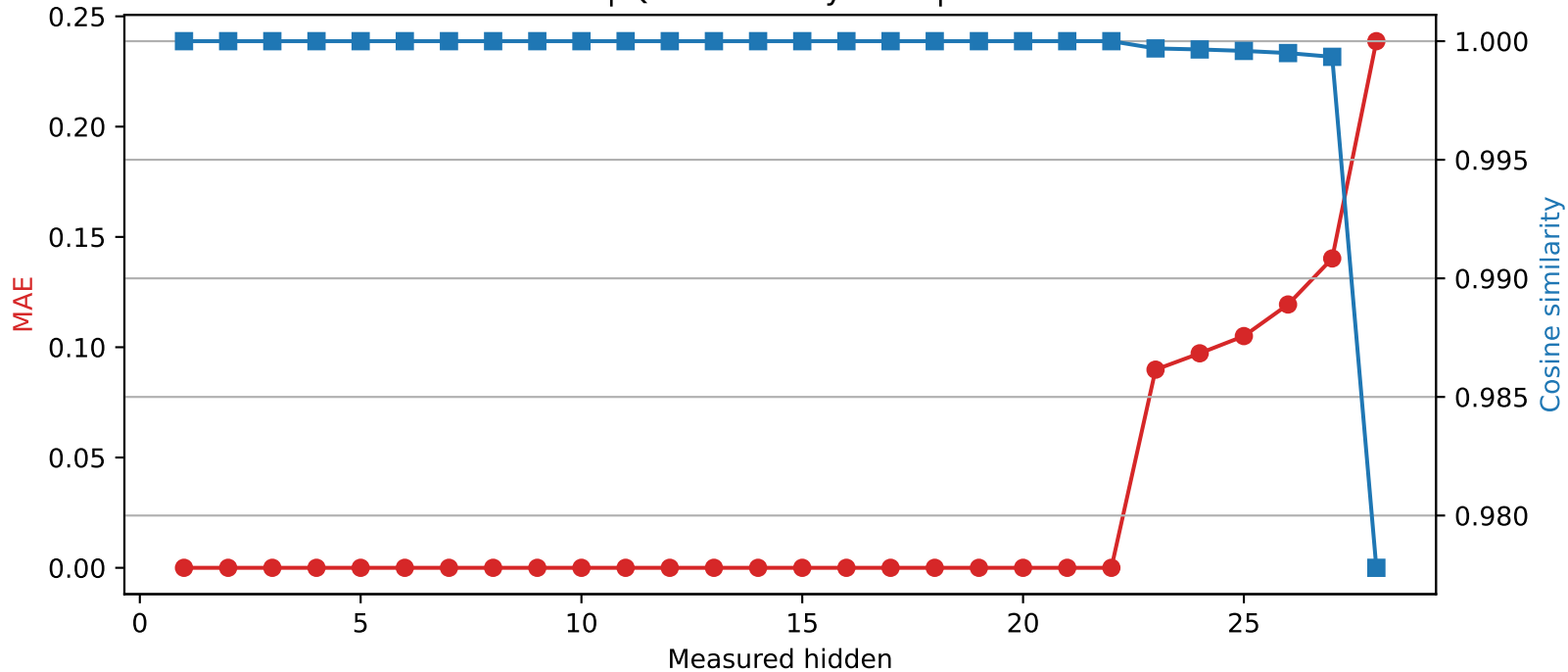
Llama-3.2-3B | Quantized layer 22 | float64 \rightarrow int2
