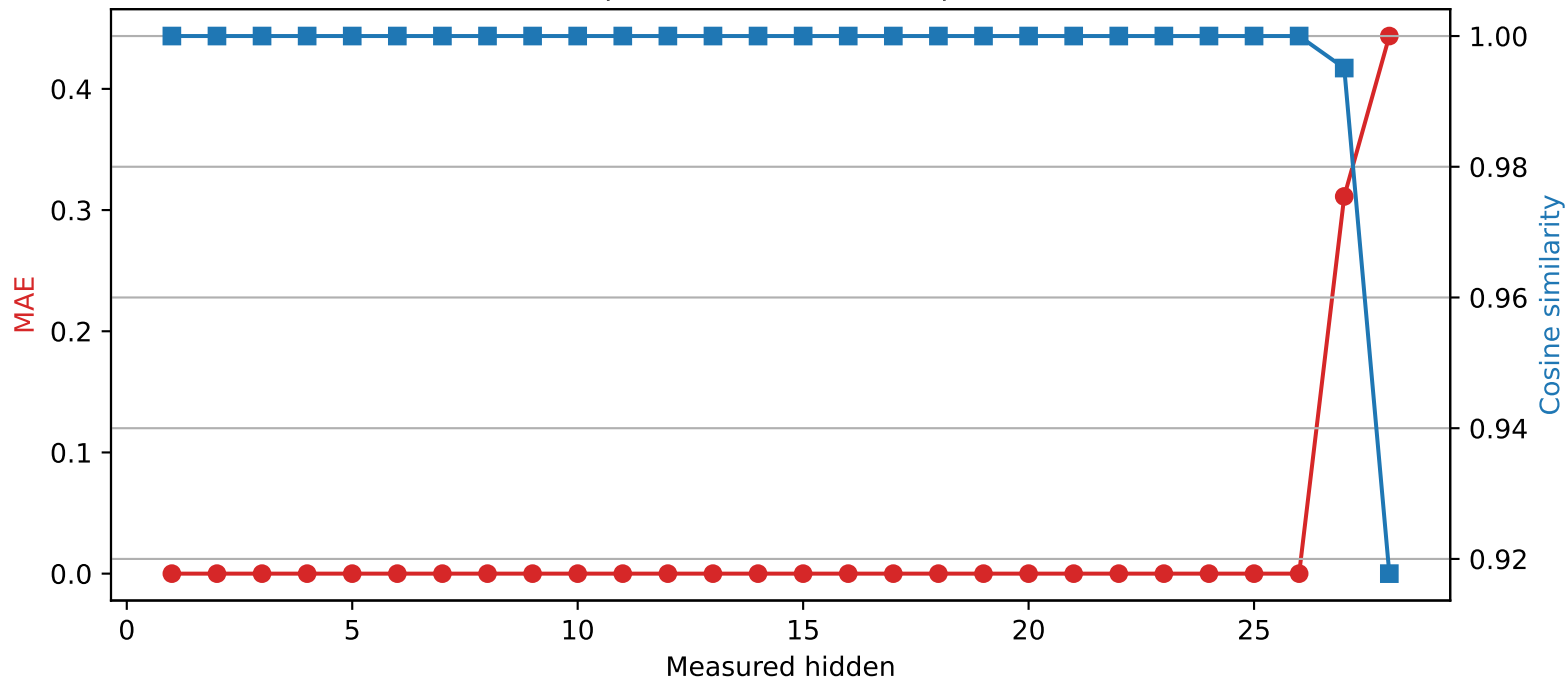
Llama-3.2-3B | Quantized layer 26 | float64 → int2
