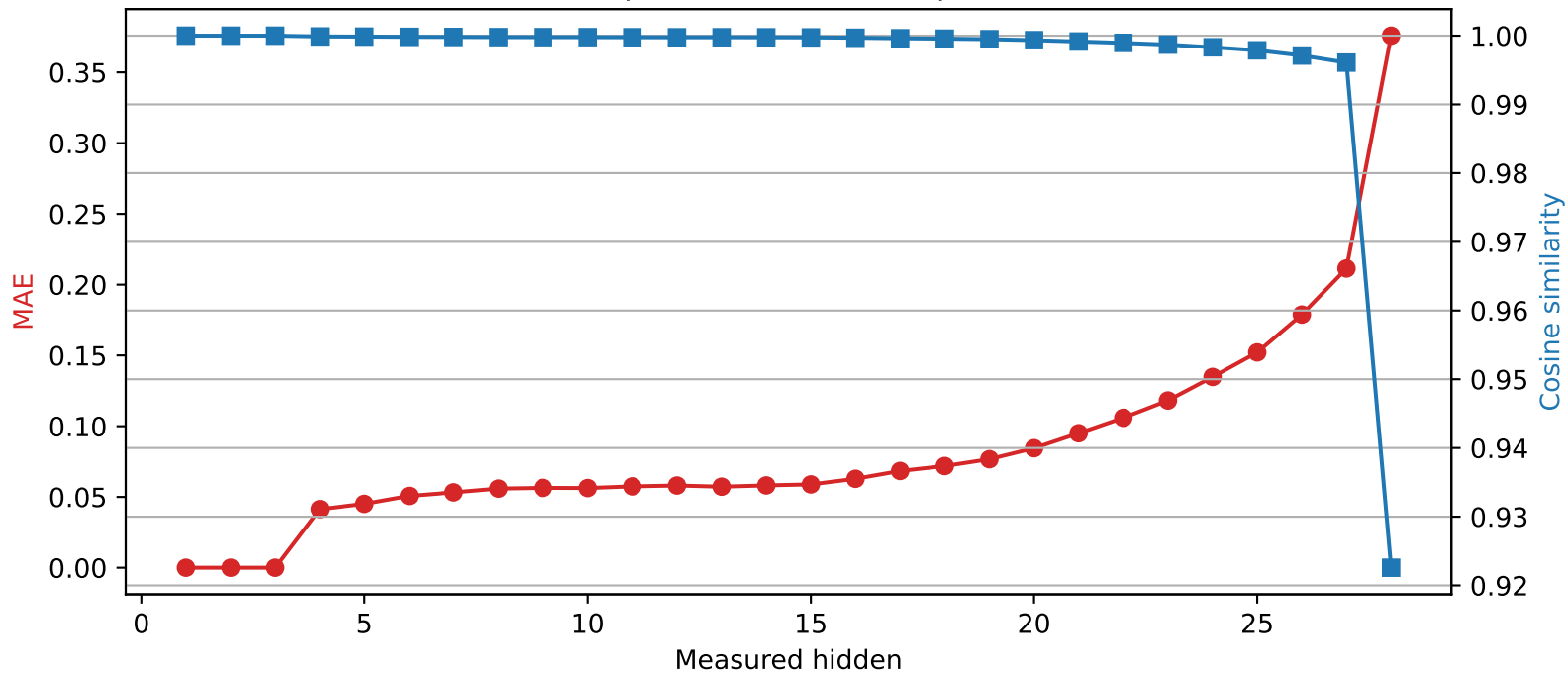
Llama-3.2-3B | Quantized layer 3 | float64 → int2
