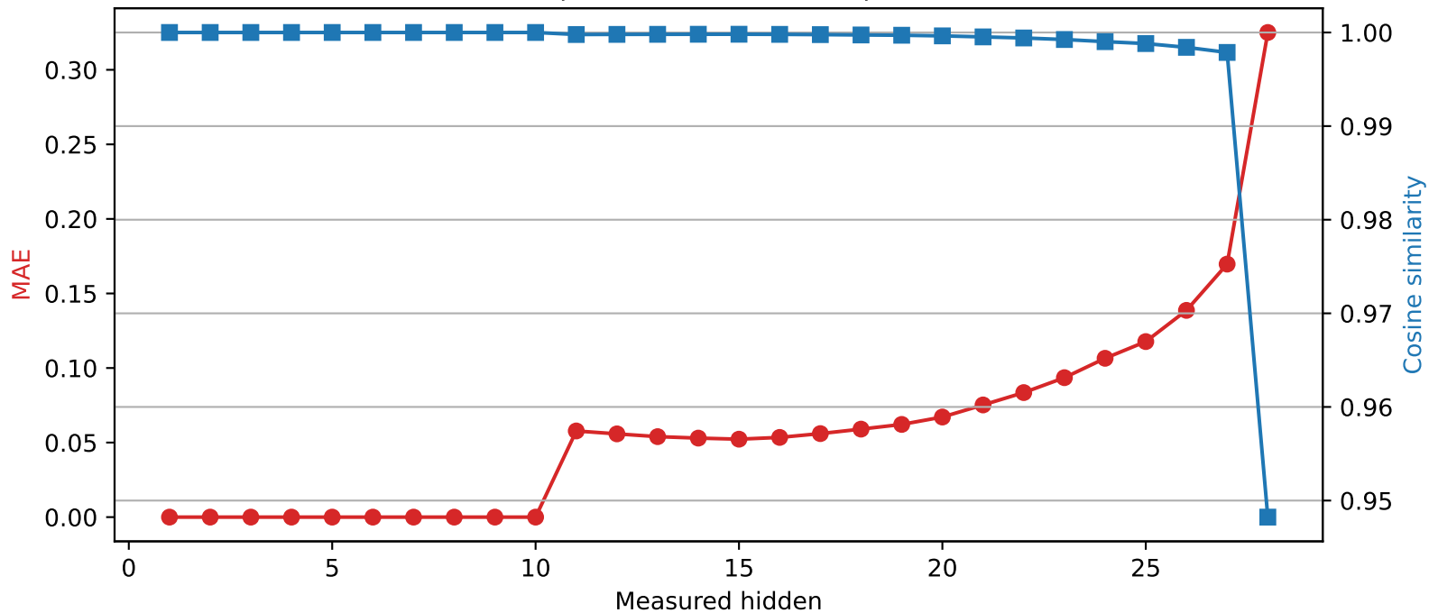
Llama-3.2-3B | Quantized layer 10 | float64 \rightarrow int2
