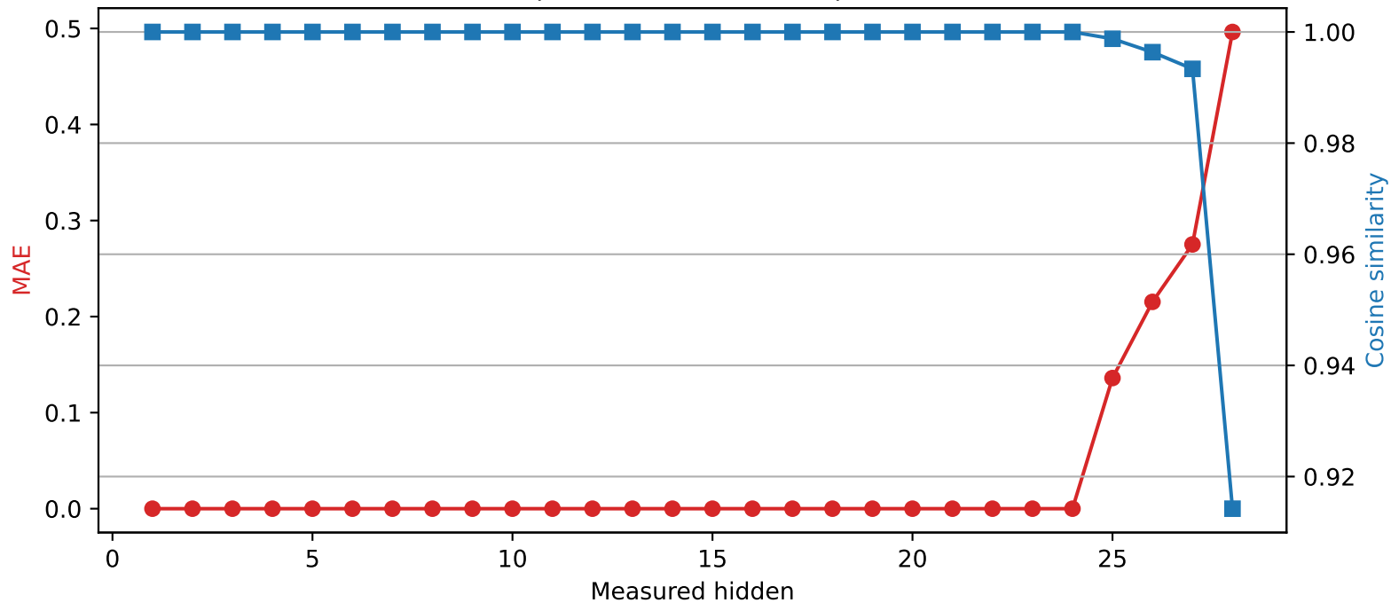
Llama-3.2-3B | Quantized layer 24 | float64 → int2
