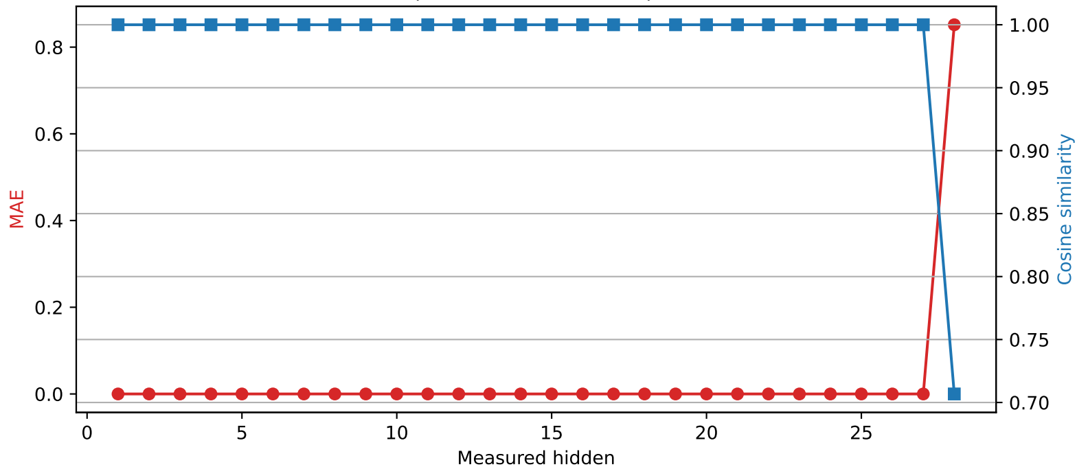
Llama-3.2-3B | Quantized layer 27 | float64 → int2
