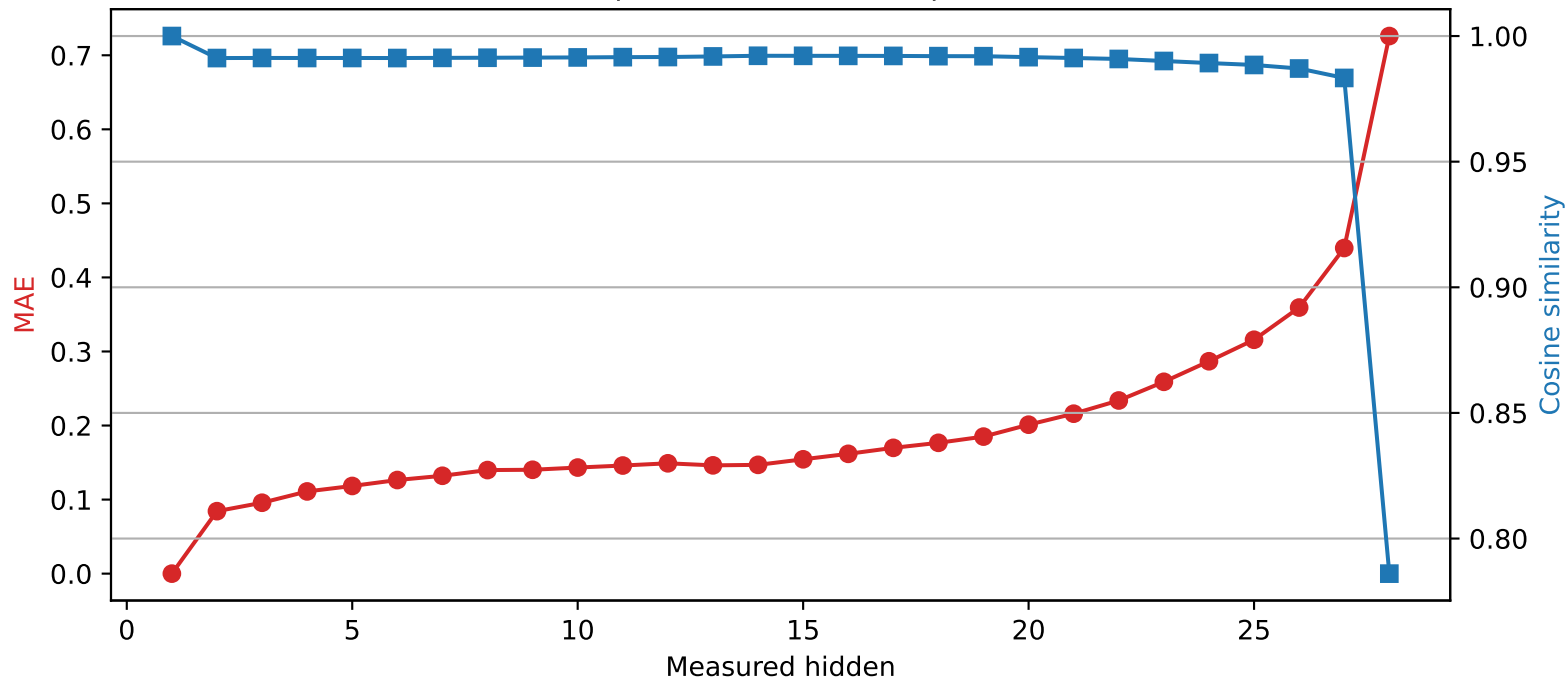
Llama-3.2-3B | Quantized layer 1 | float64 → int2
