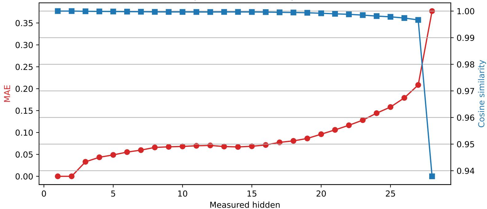
Llama-3.2-3B | Quantized layer 2 | float64 → int2
