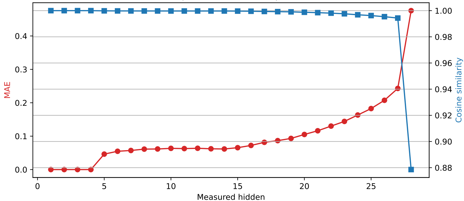
Llama-3.2-3B | Quantized layer 4 | float64 → int2
