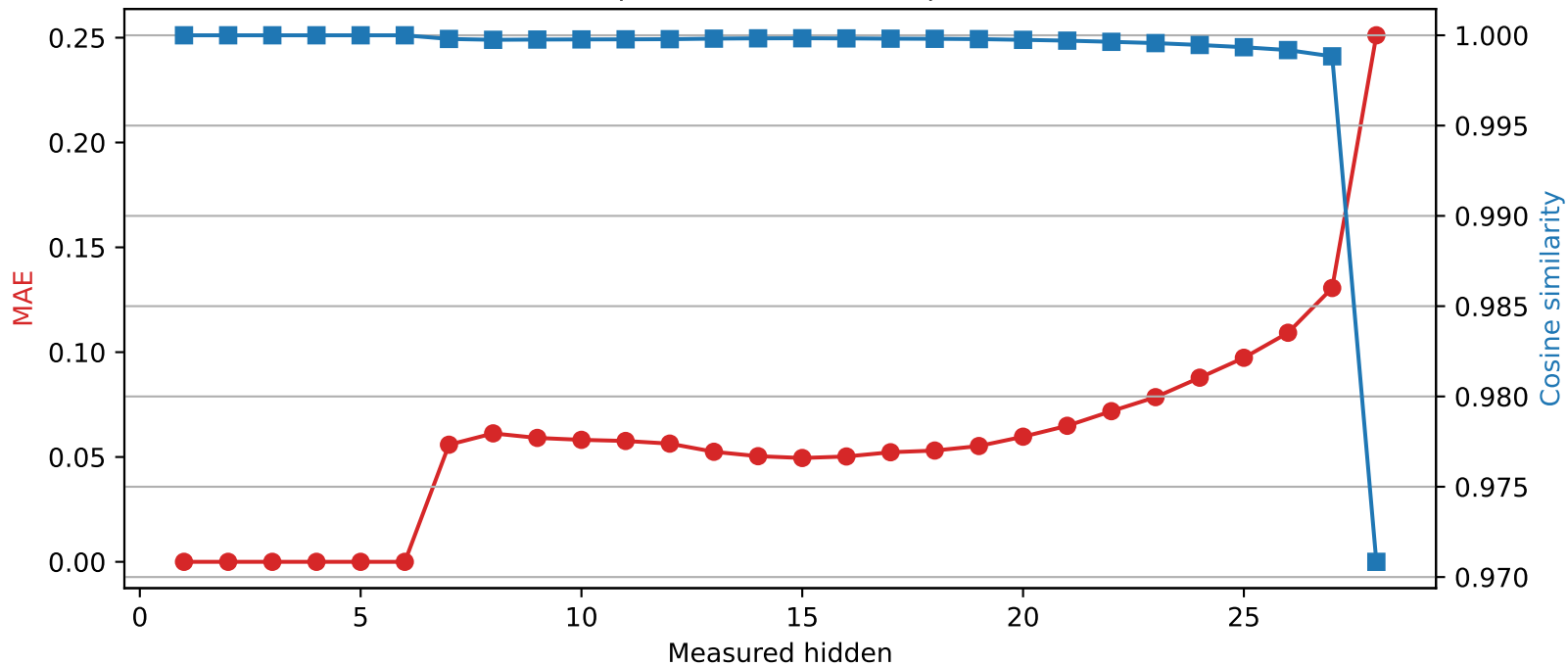
Llama-3.2-3B | Quantized layer 6 | float64 → int2
