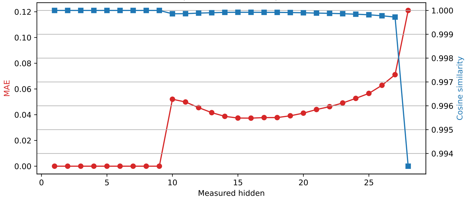
Llama-3.2-3B | Quantized layer 9 | float64 → int2
