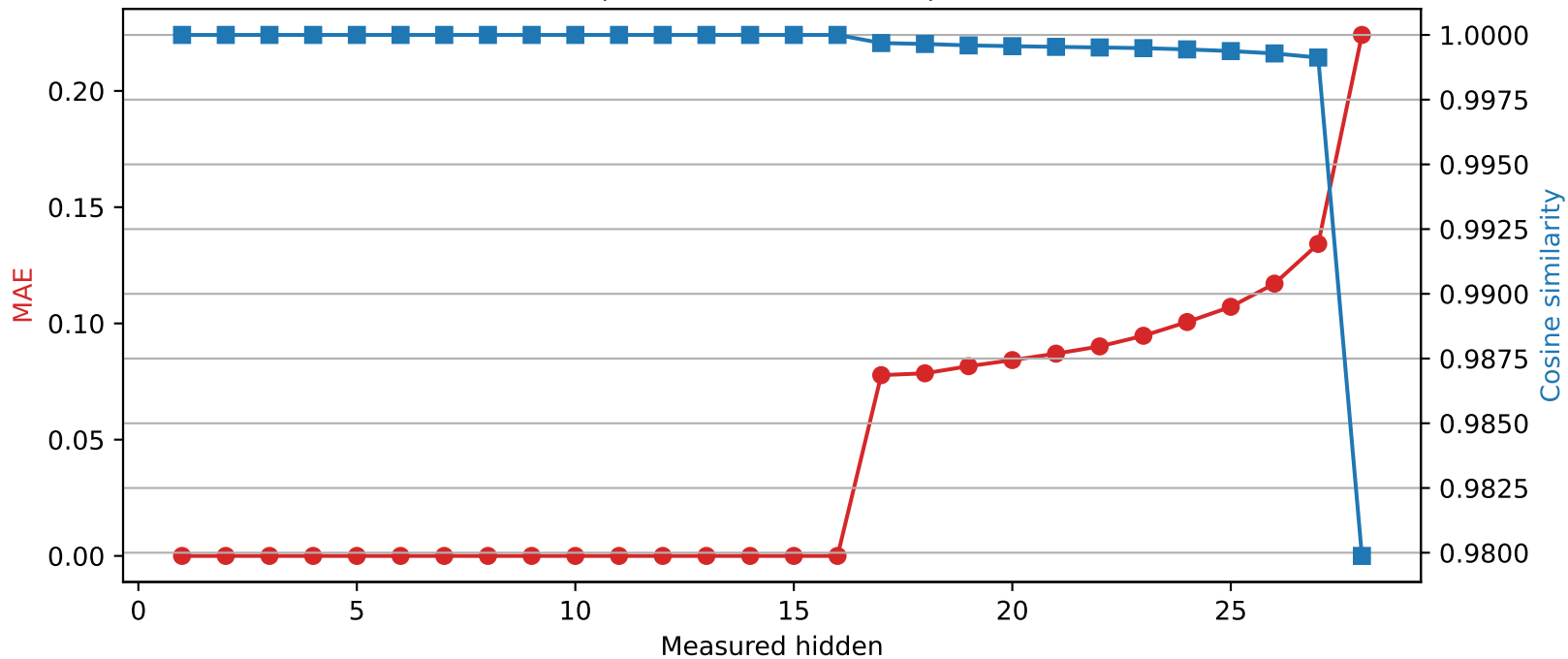
Llama-3.2-3B | Quantized layer 16 | float64 → int2
