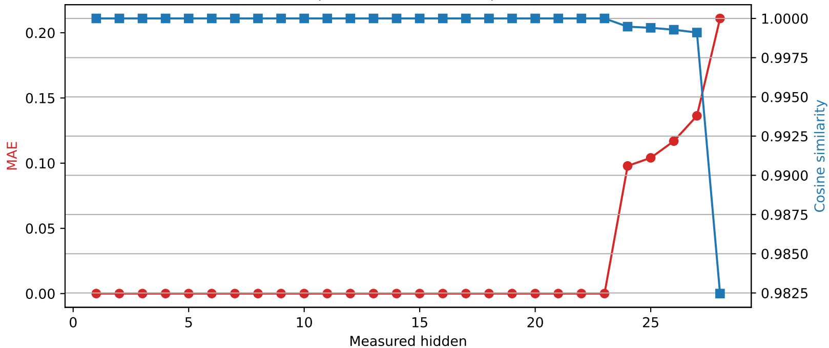
Llama-3.2-3B | Quantized layer 23 | float64 → int2
