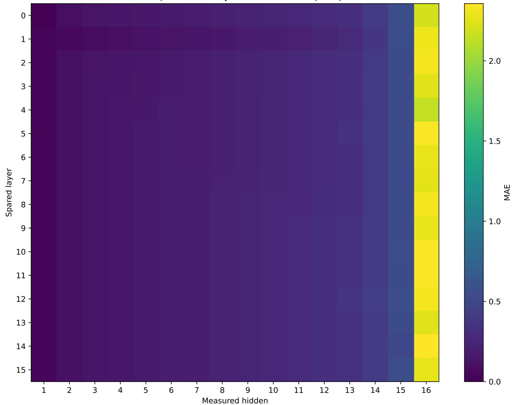
Llama-3.2-1B Mean unquantized vs hybrid MAE across 5 prompts
