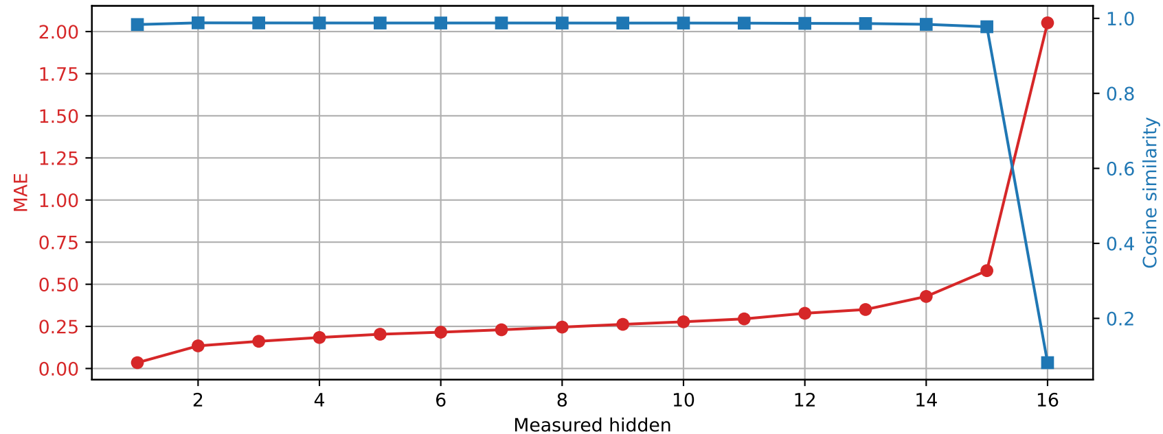
Llama-3.2-1B | Prompt 0 Unquantized vs quantized int4
