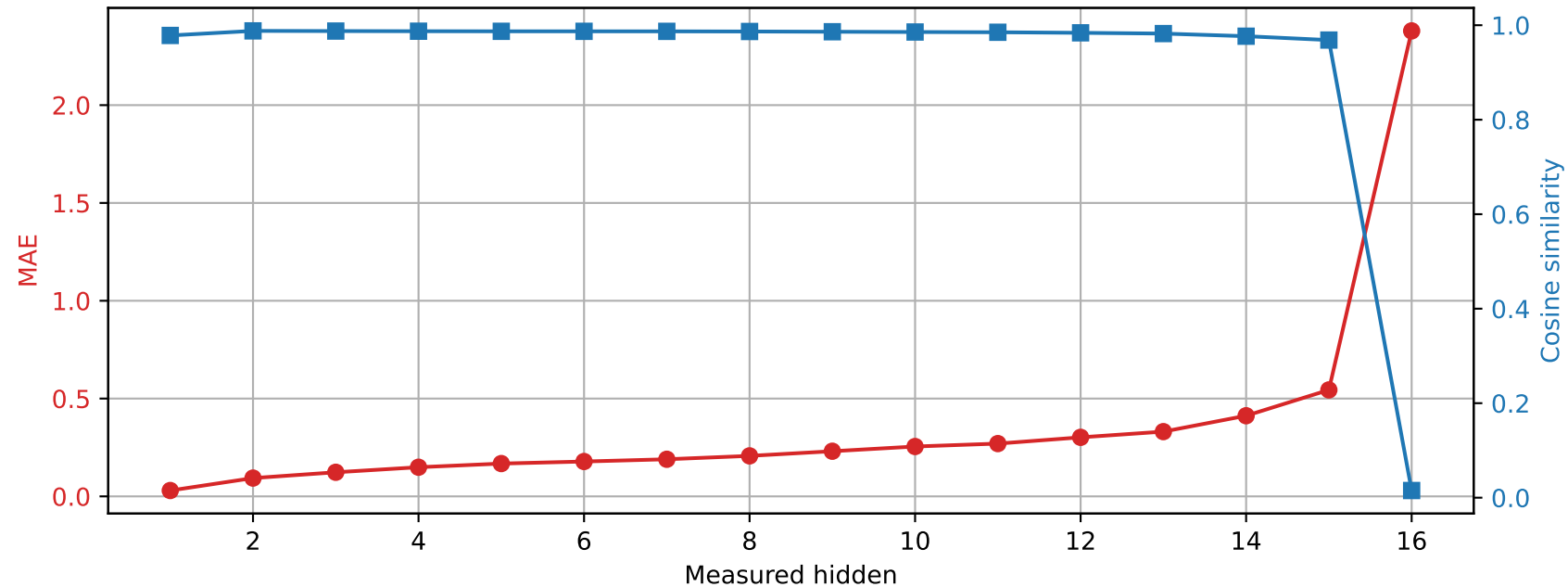
Llama-3.2-1B | Prompt 1 Unquantized vs quantized int4
