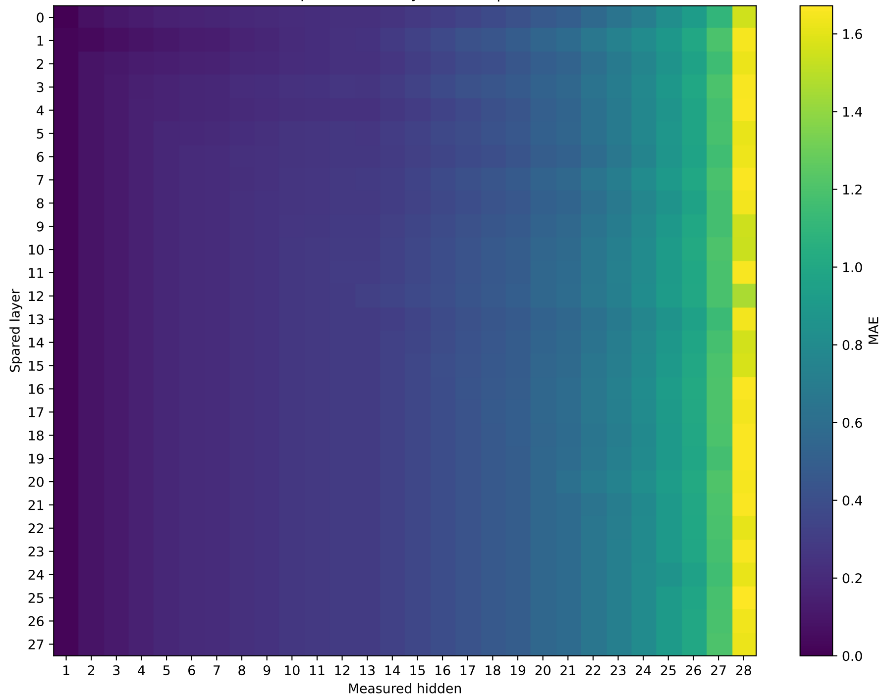
Llama-3.2-3B | Prompt 1 Unquantized vs hybrid MAE | int4
