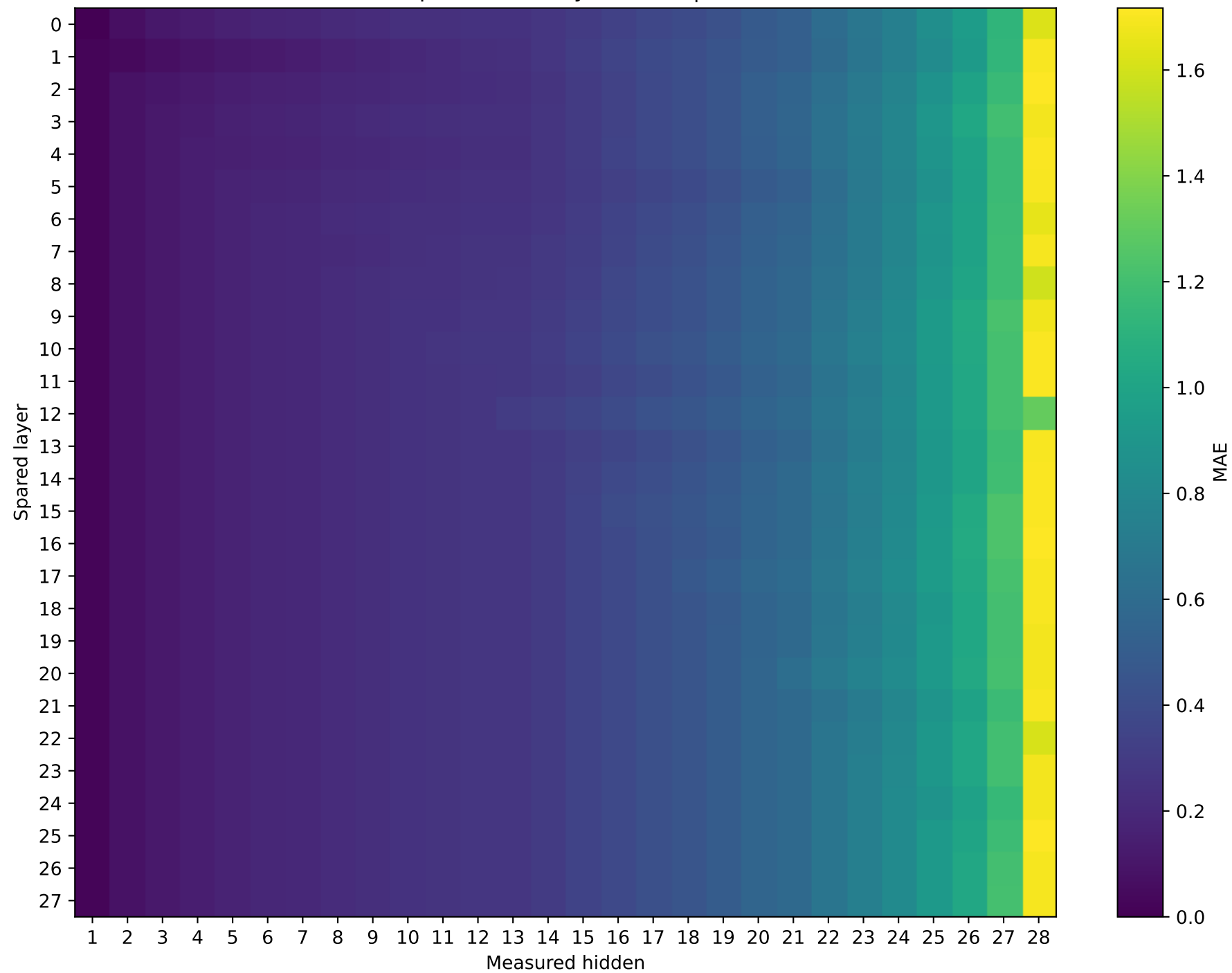
Llama-3.2-3B | Prompt 2 Unquantized vs hybrid MAE | int4
