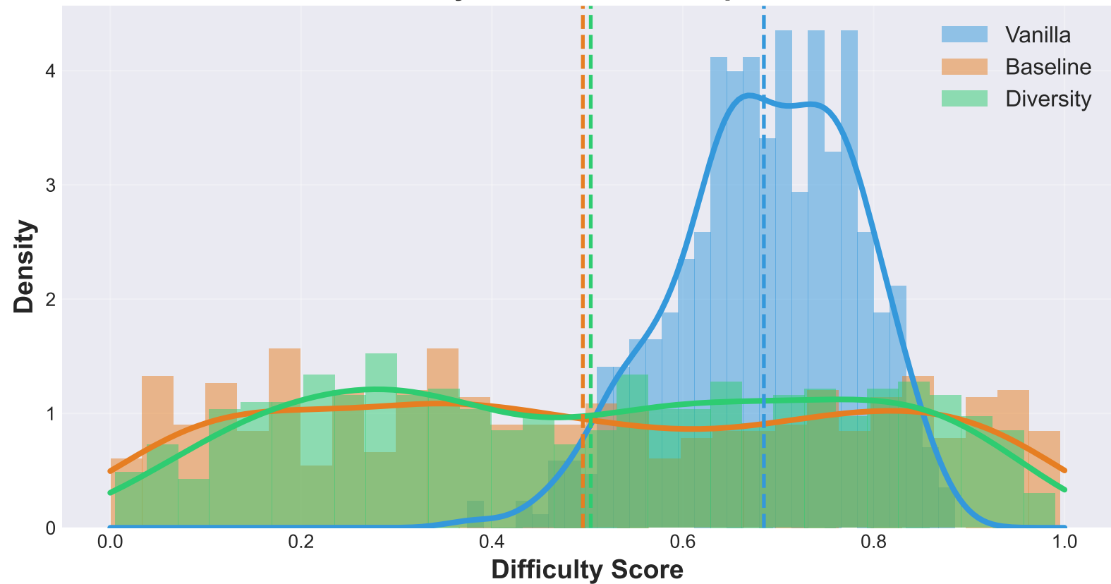
Difficulty Distribution Comparison
