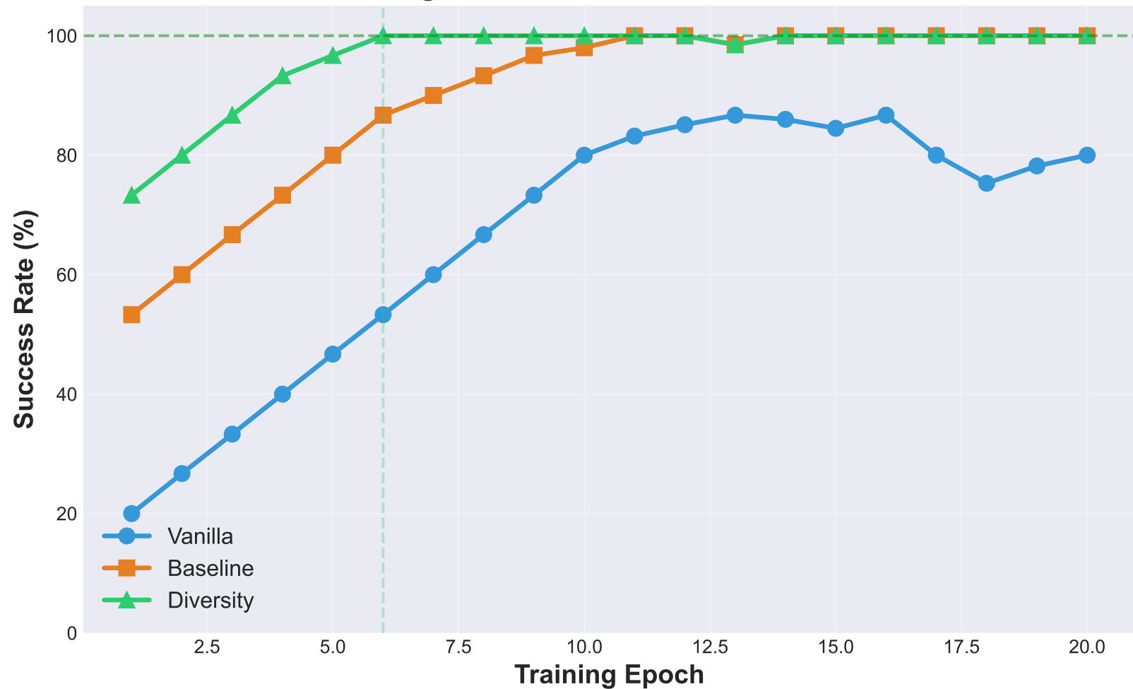
Learning Curves: Success Rate Evolution
